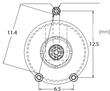
Drilling / Soldering Template
